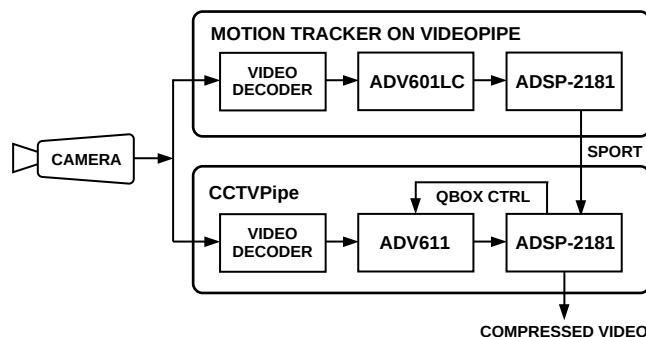
Figure 1. Two-Board Motion Tracking System
